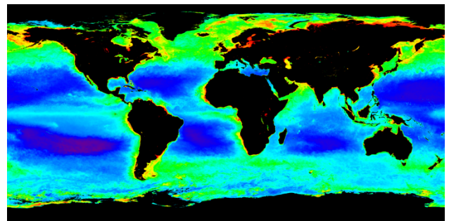
Fig. 1 Annual VIIRS-SNPP Chlorophyll Concentration in 2018, based on OCx Algorithm, download from NASA website.
