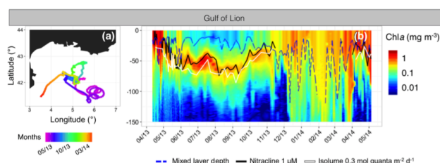
Fig.2 (a) Trajectory and (b) Profiles of chlorophyll concentration versus time for the float deployed in the Gulf of Lion [5].
